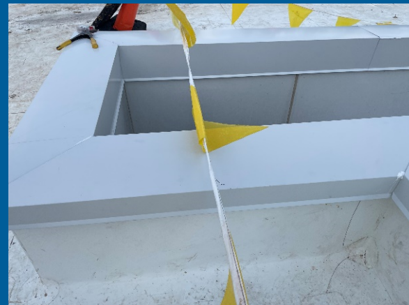
Rooftop Coping Installed
